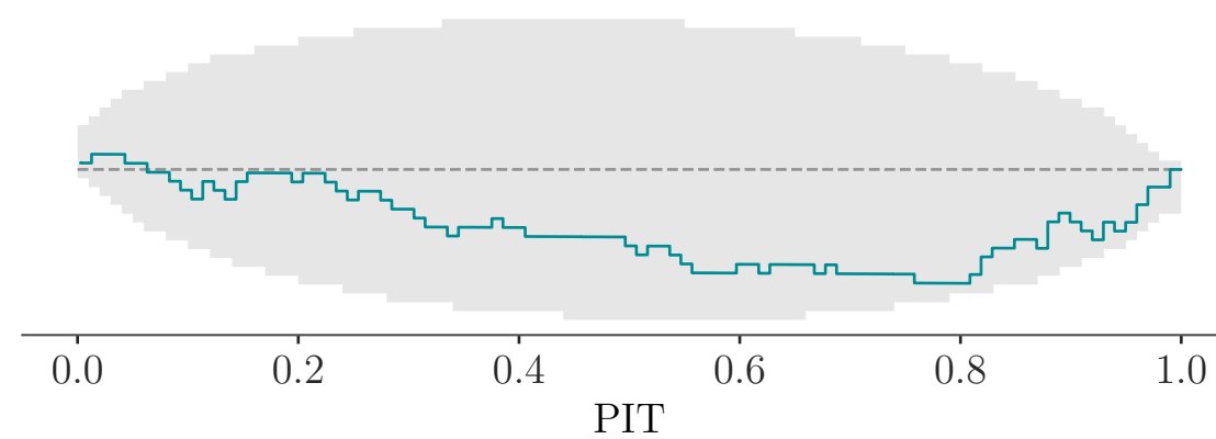
log_Ne_a (corrected)
