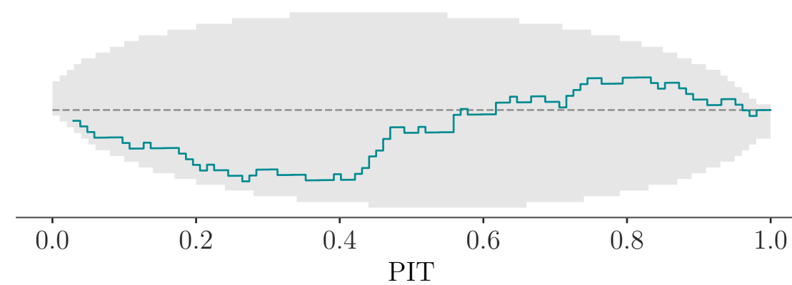
log_t0 (corrected)
