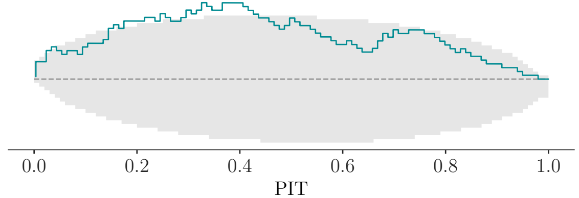
\log_{\text{Ne\_a}} (approximate)
