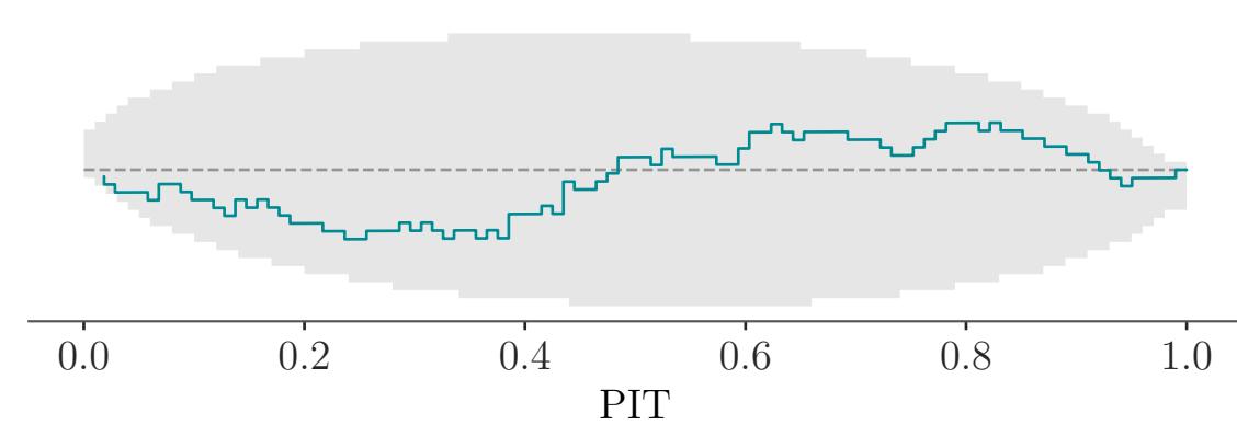
\log_{\text{t0}} (approximate)
