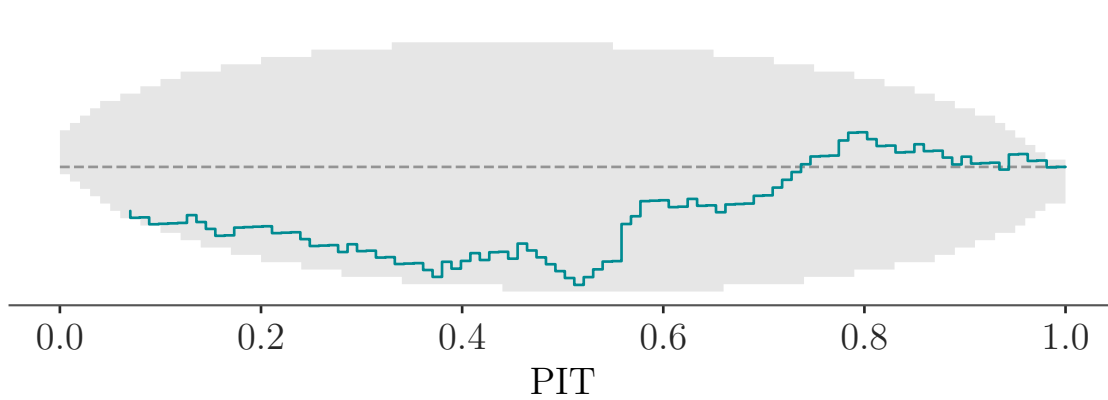
log_Ne_c (uncorrected)
