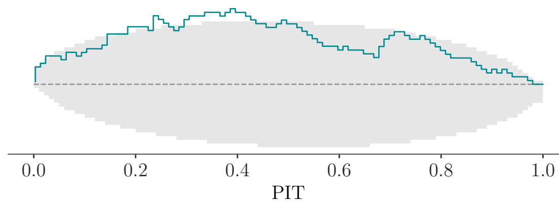
log_Ne_a (uncorrected)
