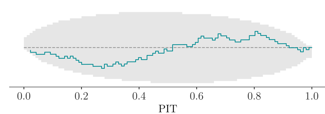
log_t0 (uncorrected)
