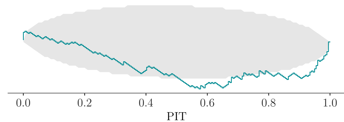
\log_{t0} (approximate)
