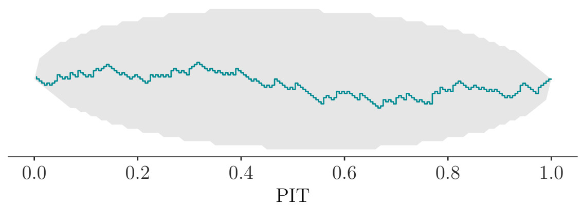
\log_{\text{Ne}_a} (approximate)
