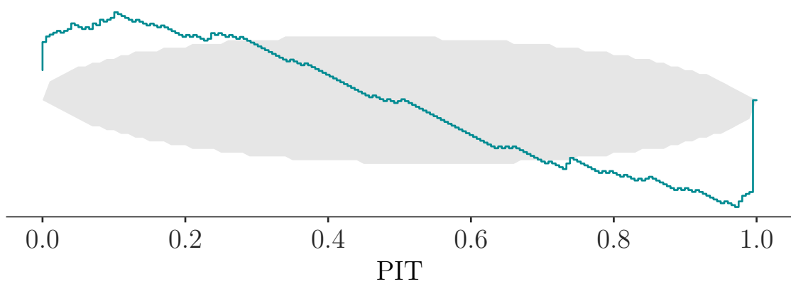
log_Ne_c (approximate)
