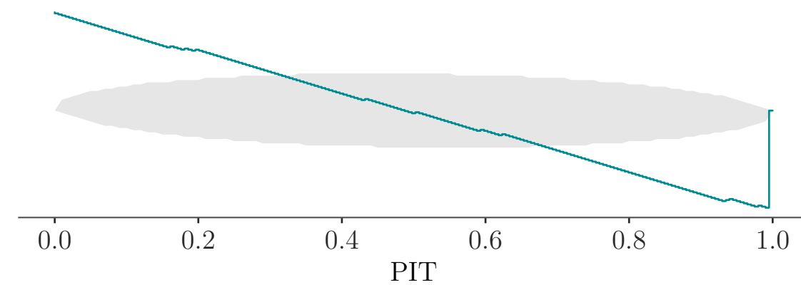
log_Ne_a (corrected)
