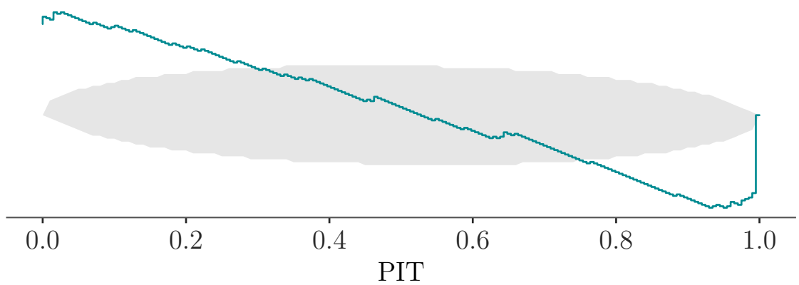
log_Ne_c (corrected)
