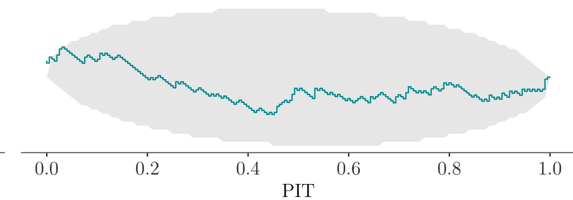
log_t0 (corrected)
