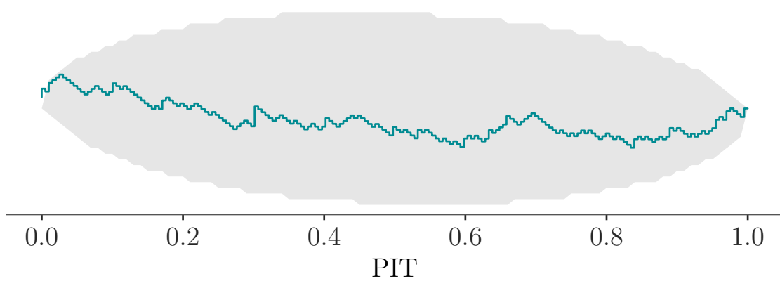
log_t0 (corrected)
