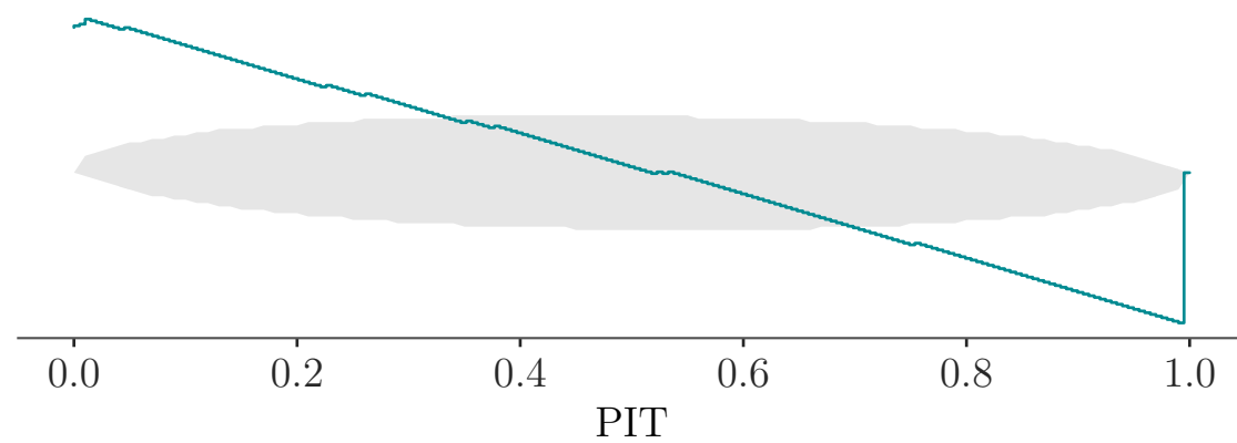
log_Ne_a (corrected)
