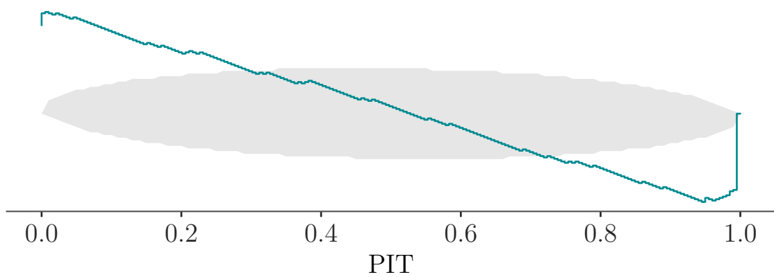
log_Ne_c (corrected)
