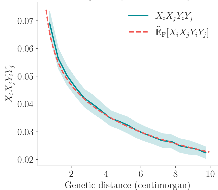
Linkage disequilibrium decay
