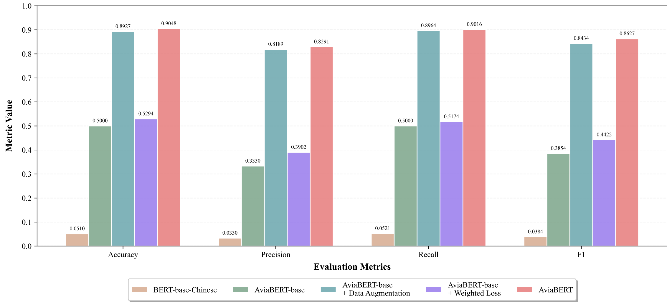
Comparison of Five Models on Different Evaluation Metrics
