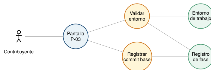
Figura 22: Diagrama de robustez de CU-001-001 — Onboarding.
