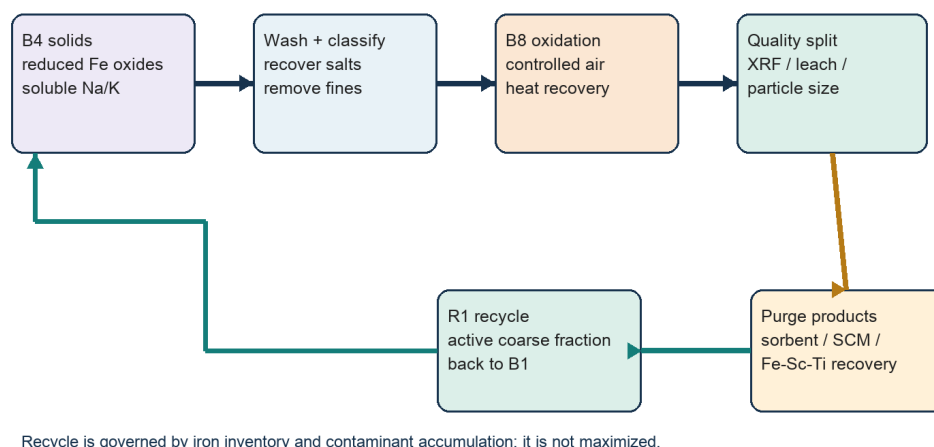
Figure 4.5. B8 conditioning, controlled purge, and R1 recycle. Recycle is governed by iron inventory and contaminant accumulation; it is not maximised.
