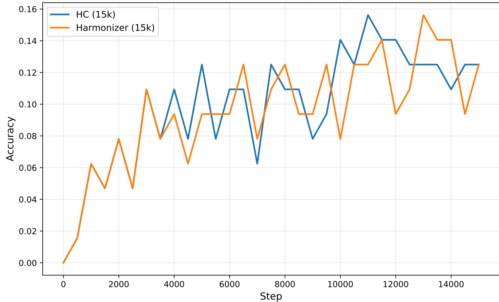
KV Retrieval Accuracy vs Step
