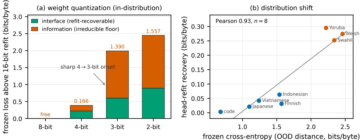
Figure 11: External replication on Pythia-410m: the two failure modes the paper isolates on systems with exact ground truth, separated by the same frozen-versus-refit pair. (a) Weight quantization (in-distribution; bits/byte above the 16-bit head-refit reference). Each bar splits the frozen loss into the head-refit-recoverable interface part and the irreducible information-borne floor; the floor jumps sharply between 4 and 3 bits, the information-borne signature. (b) Distribution shift across eight Latin-script corpora: head-refit recovery versus frozen cross-entropy (an OOD-distance proxy). Recovery is near zero for in-distribution/mild shifts and grows with OOD distance, the interface-borne signature (Pearson 0.93, n = 8 ). Values are the verified numbers of Tables 4 and 5.
