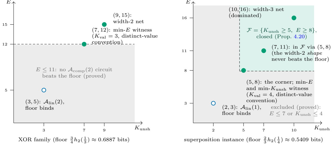
Figure 4: The payment frontier (Definition 4.13), one panel per family; axes are unshared stored-parameter counts K_{\text{unsh}} (Section 2.4) and per-evaluation operations E under the Section 4.1 conventions; the parenthetical K_{\text{val}} notes report the same witnesses under the different, distinct-value convention. Filled circles: budgets at which an affine-threshold composition provably beats the linear floor to H = 0 (Thm. 4.4, Props. 4.14 and 4.19, Thm. 4.5(iv)); open circles: budgets at which the floor provably binds (Prop. 4.12). Left: for XOR the shaded region E \leq 11 is exhaustively excluded and the minimal- E edge sits exactly at E = 12 (Prop. 4.14); the E = 15 point is the hidden-layer threshold-ladder witness, the E = 12 point cheaper because \mathcal{A}_{\text{comp}}(2) allows the second gate to read both raw coordinates and the earlier gate’s output (Remark 4.15); the K_{\text{unsh}} structure off the known points belongs to the residue (Open Problem 4.22(i)). Right: the superposition panel is closed (Prop. 4.20): the frontier is exactly the quadrant \mathcal{F} = \{K_{\text{unsh}} \geq 5, E \geq 8\} , its corner attained by the Prop. 4.19 witness, every budget outside it excluded, and the budget point (7, 11) in \mathcal{F} even though the width-2 network shape priced there never beats the floor (Thm. 4.5(iii), Remark 4.21).
