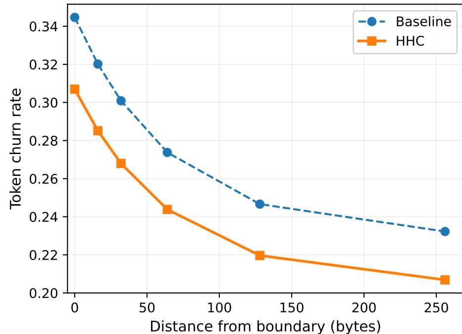
(a) Token Churn vs Distance
