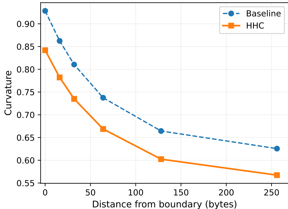
(b) Curvature vs Distance
