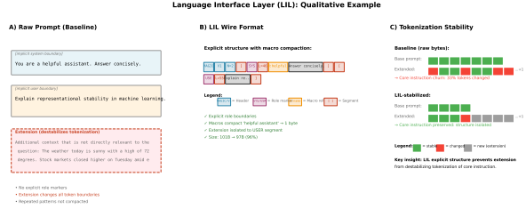
Figure 3: Qualitative example illustrating the Language Interface Layer (LIL). Panel A shows a raw prompt with repeated scaffolding and implicit role boundaries. Panel B shows the reversible LIL wire format with explicit role markers (SYS, USR) and macro-compacted interface patterns (M:helpful_a replaces “You are a helpful assistant”). Panel C demonstrates that extending the prompt does not destabilize tokenization of the core instruction under LIL: the system segment tokens remain stable (green) while extension tokens are isolated, whereas baseline representations exhibit churn (red) throughout.
