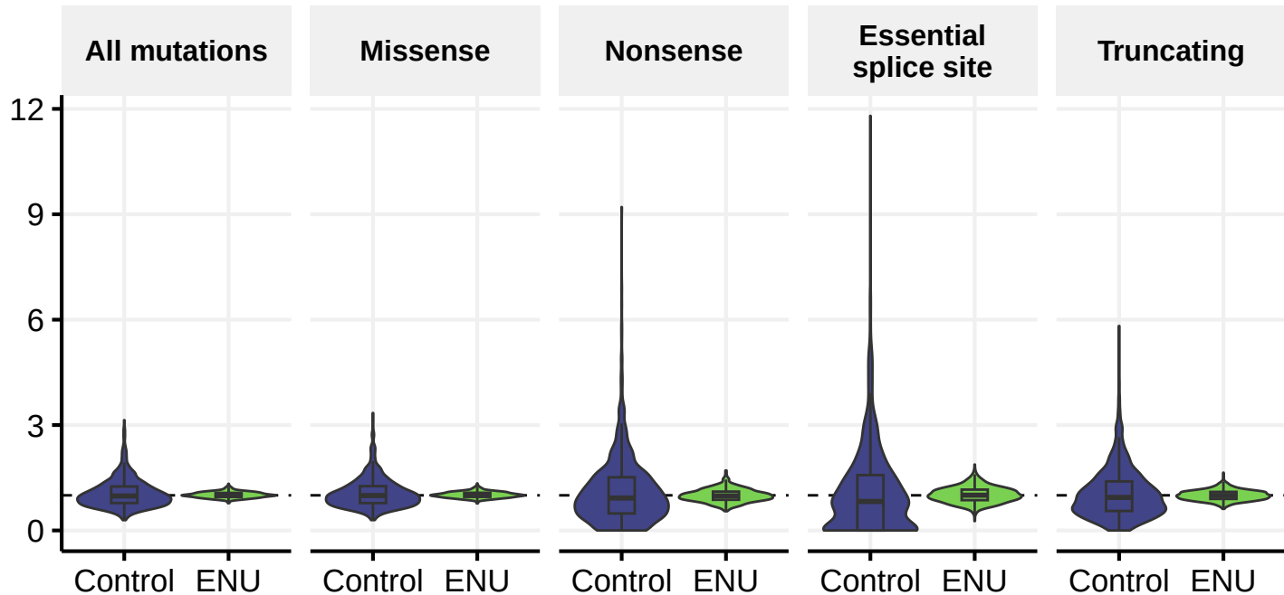
Global dN/dS Ratio
