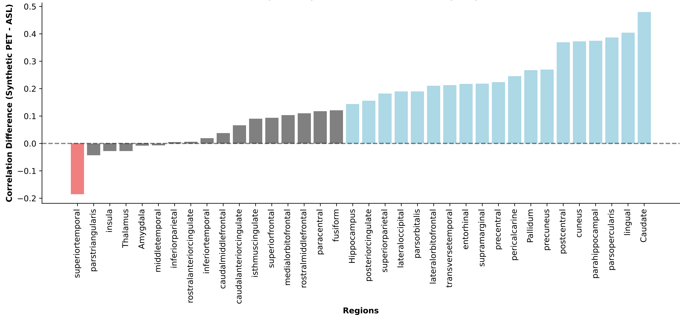
TLE - Asymmetry Correlation Difference by Region
