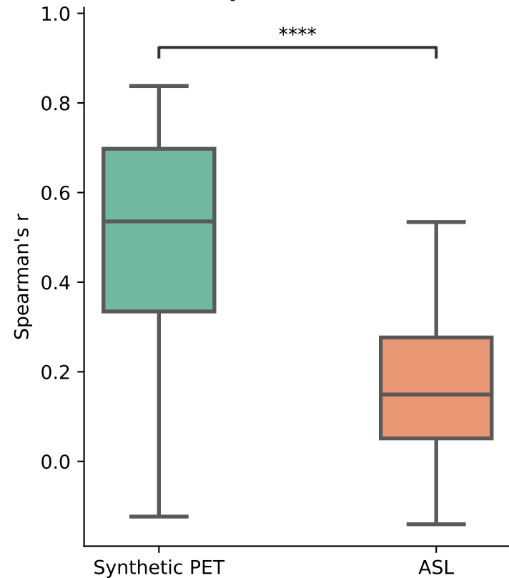
Spearman's r
