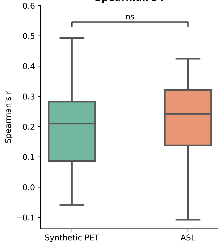
Spearman's r
