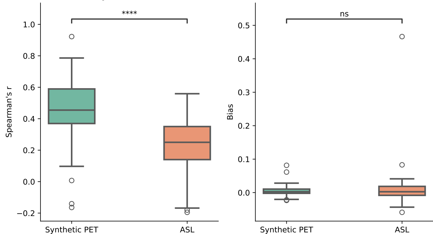
Spearman's r
