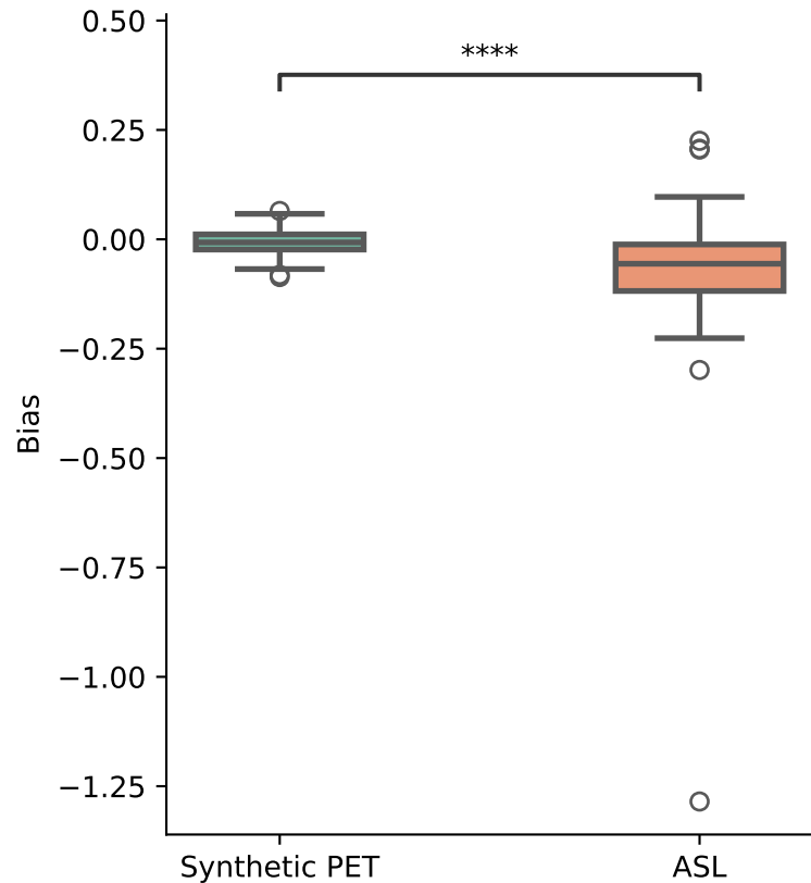
Bias
