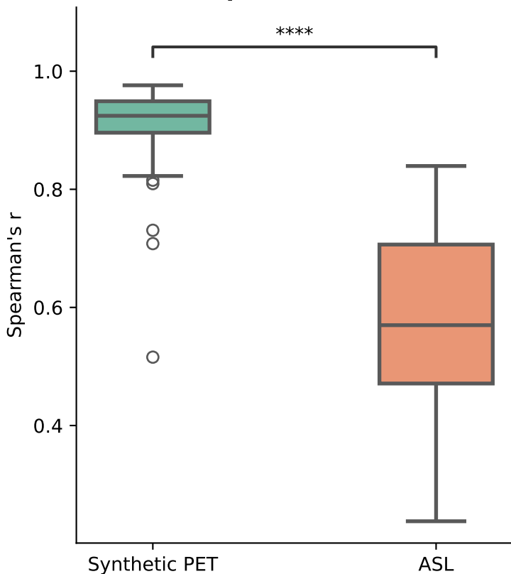
Spearman's r
