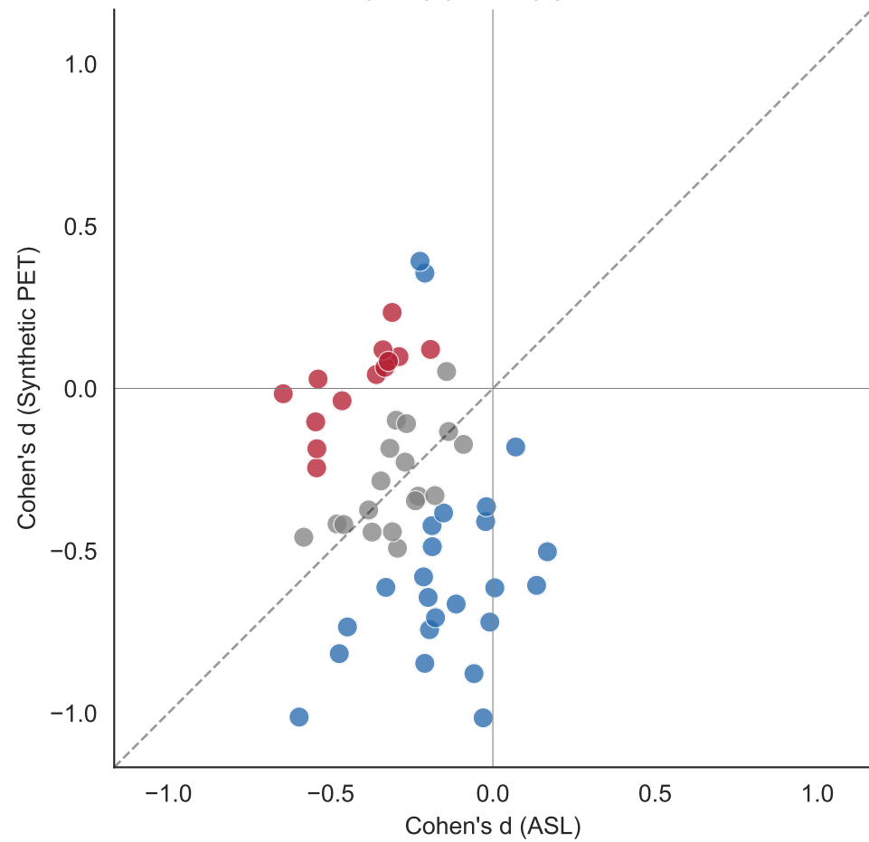
MCI - HarvardOxford (cross-validated) improvement-corr r=0.85 ( p=3.19\text{e-}16 ) Synth |d| > \text{ASL } |d| : 31/55
