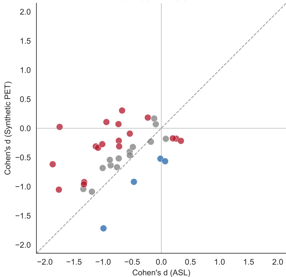
MCI - DKT (cross-validated) improvement-corr r=0.91 ( p=3.15\text{e-}16 ) Synth |d| > \text{ASL } |d| : 18/41
