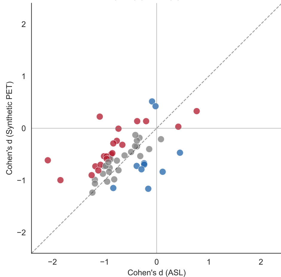
MCI - HarvardOxford (cross-validated) improvement-corr r=0.85 ( p=3.19\text{e-}16 ) Synth |d| > \text{ASL } |d| : 31/55
