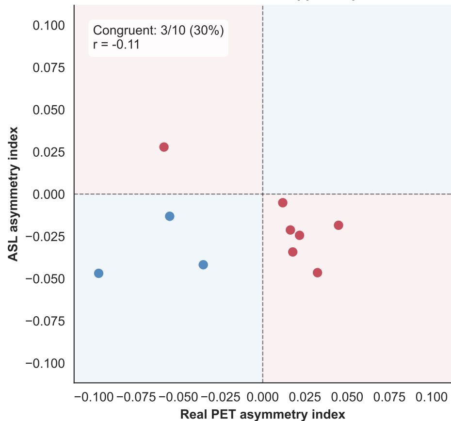
Real PET vs ASL — hippocampus
