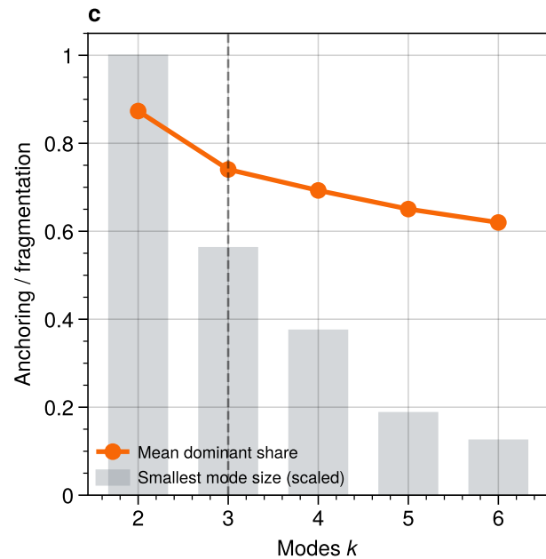
Anchoring stays interpretable before modes fragment
