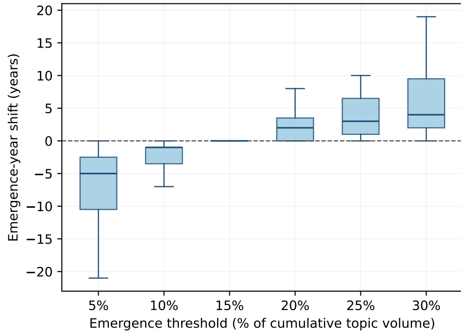
Shift Relative to 15% Baseline
