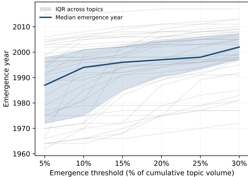
Topic Emergence Year vs Threshold
