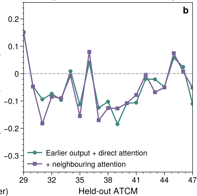
The gain recurs across held-out meetings
