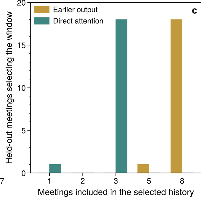
Forecasts select long output memory, recent attention
