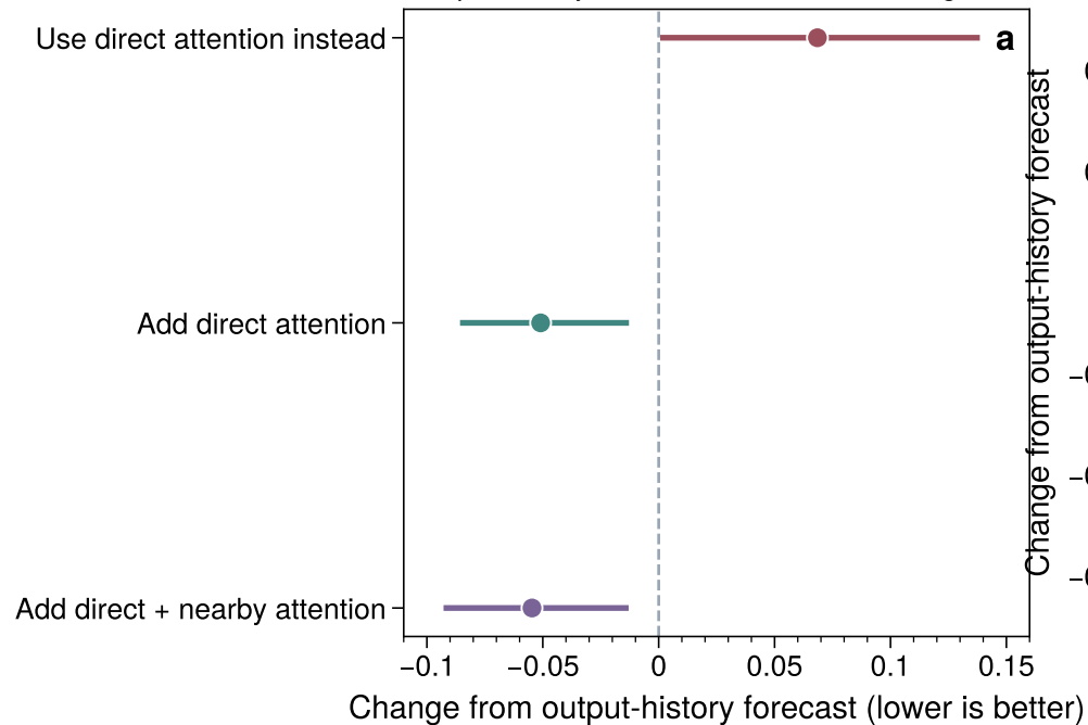
Output history and direct attention work together
