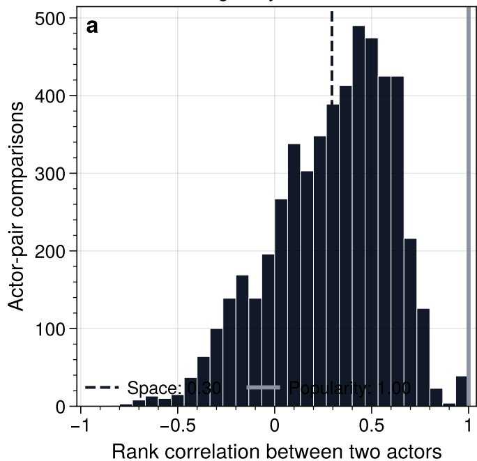
Rankings vary across actors
