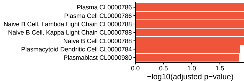
cluster_7
