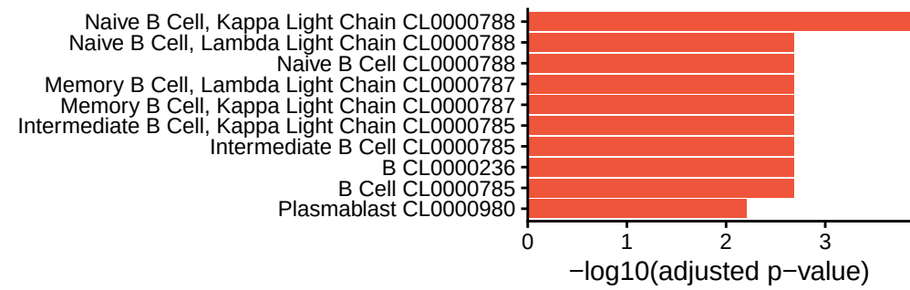
cluster_4
