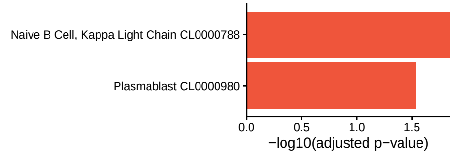
cluster_8
