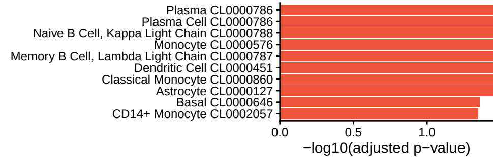
cluster_6
