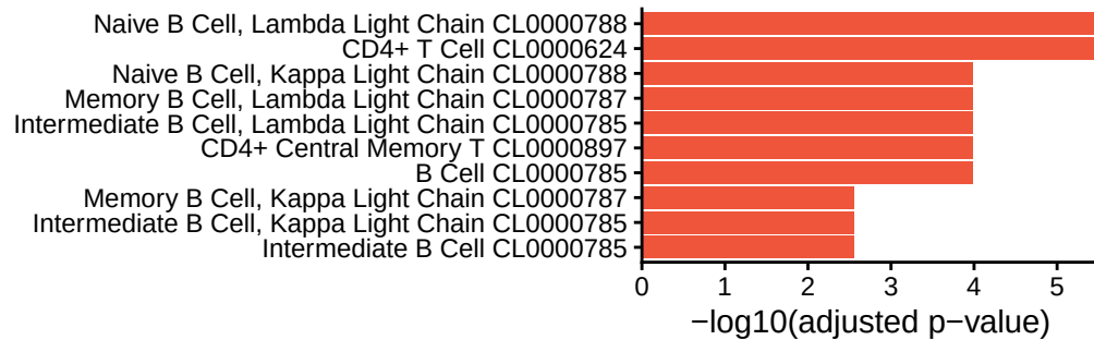
cluster_7
