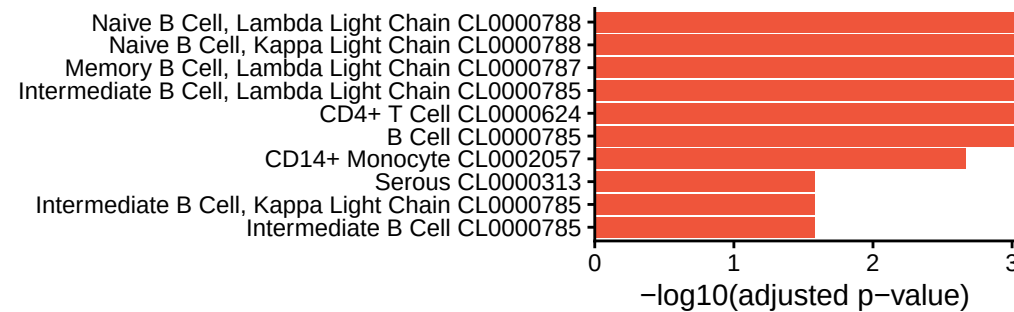
cluster_8
