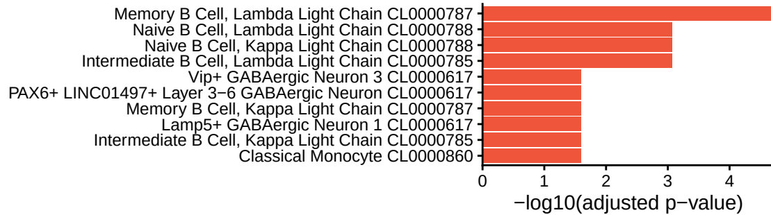
cluster_5
