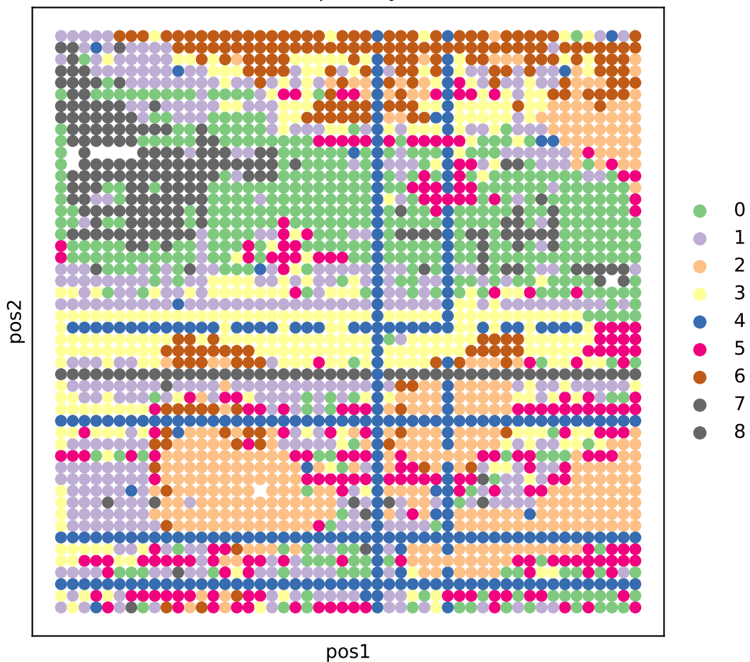
Leiden RNA (Spatially Embedded)
