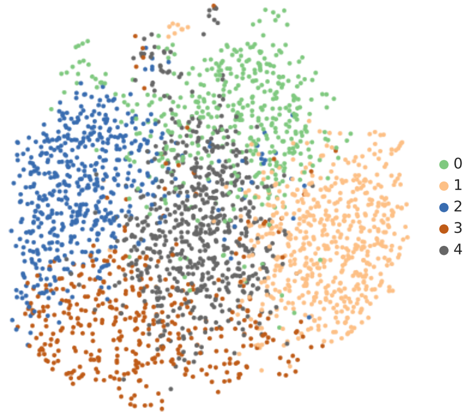
K-means
