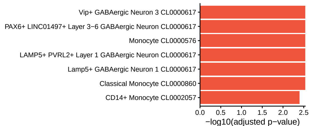
cluster_7
