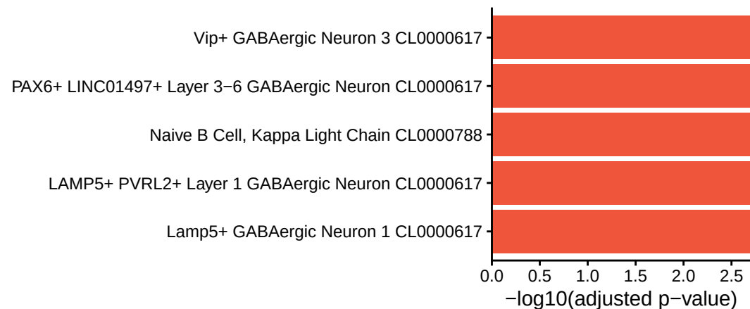
cluster_4
