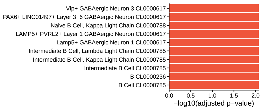
cluster_6
