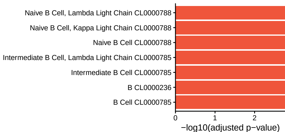
cluster_6
