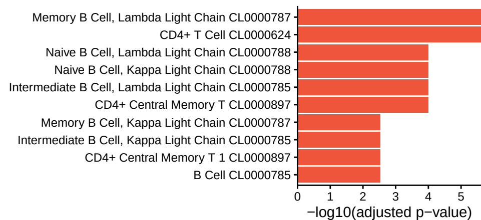
cluster_7
