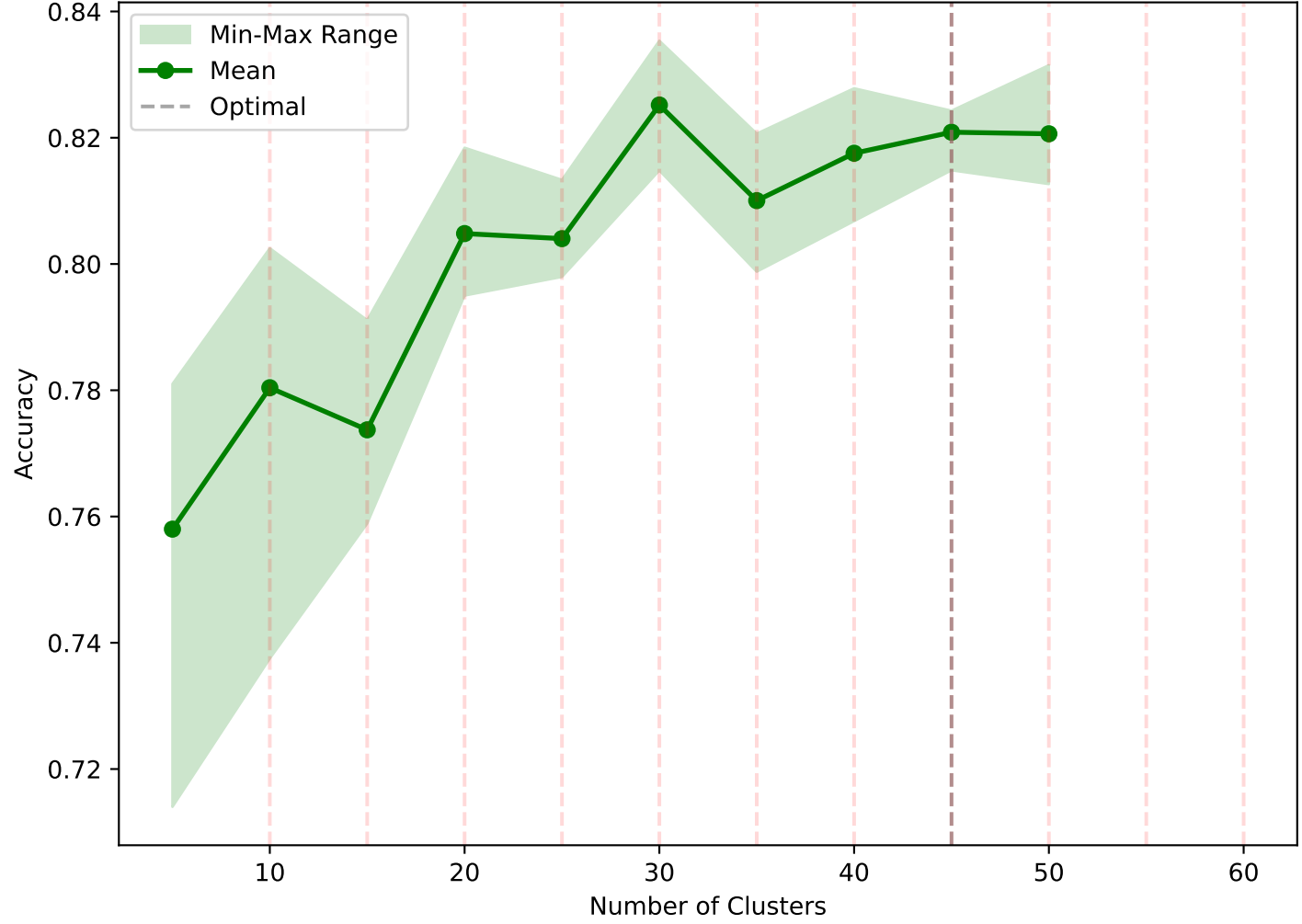
Autograder Accuracy vs. Number of Clusters
