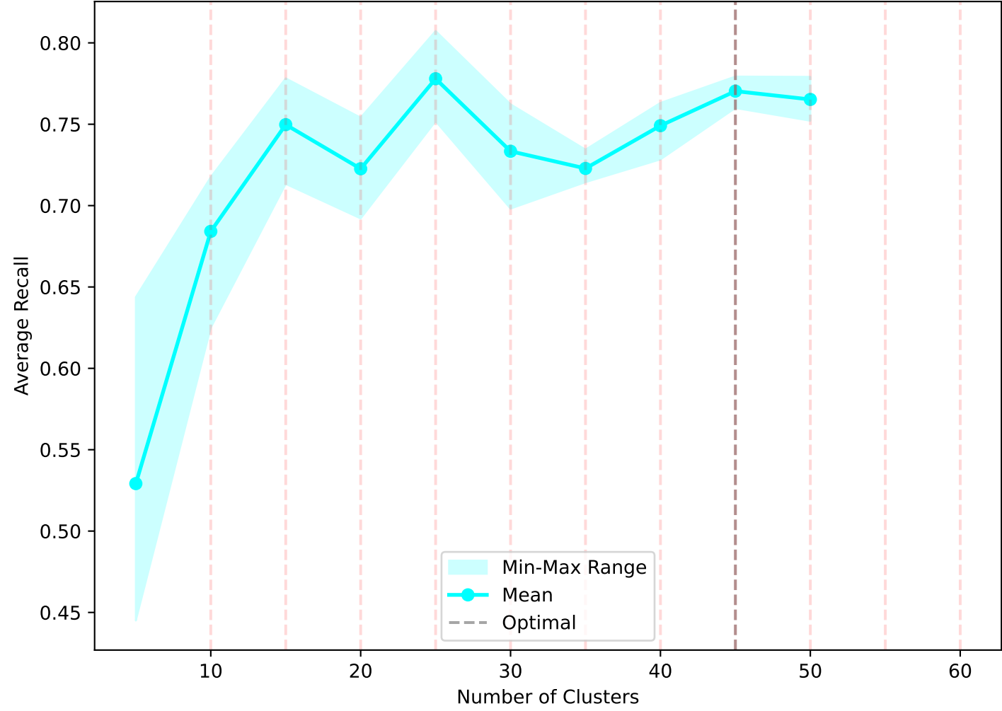
Average Recall vs. Number of Clusters
