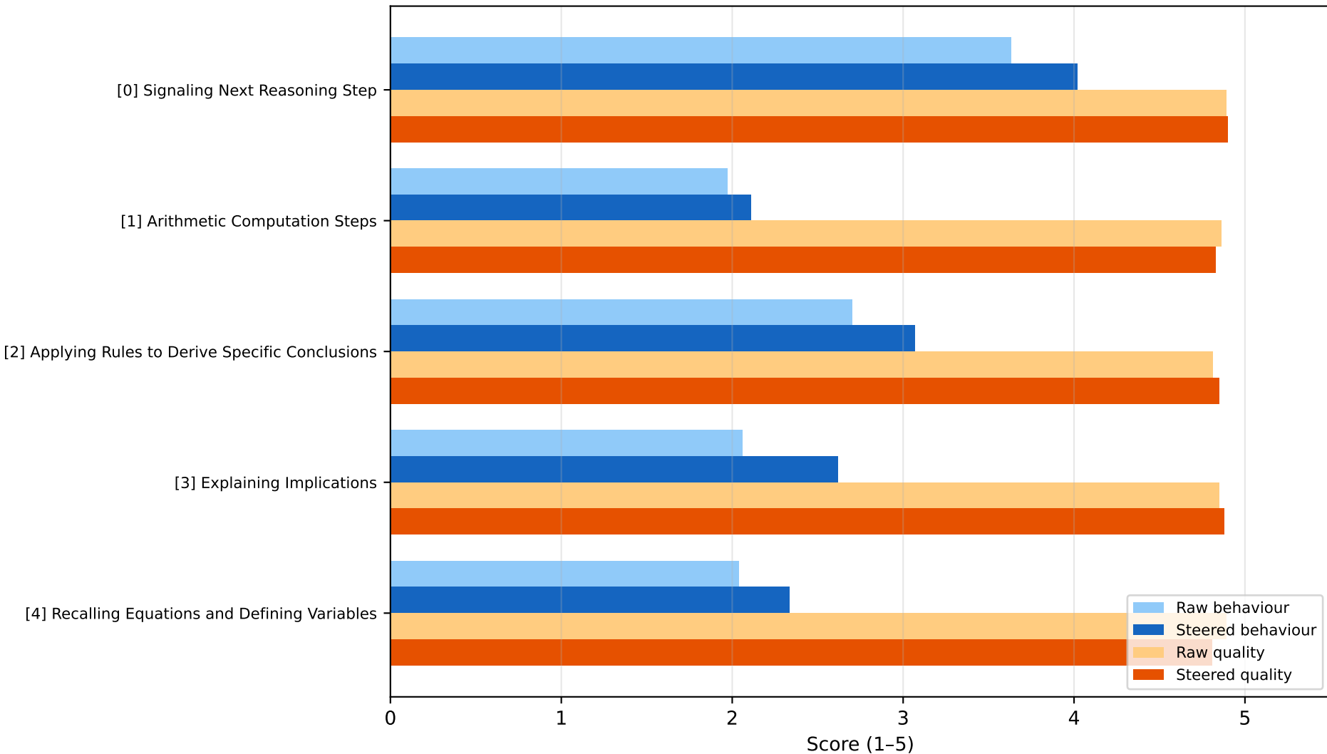
Steering Effectiveness: all categories (best coeff)
