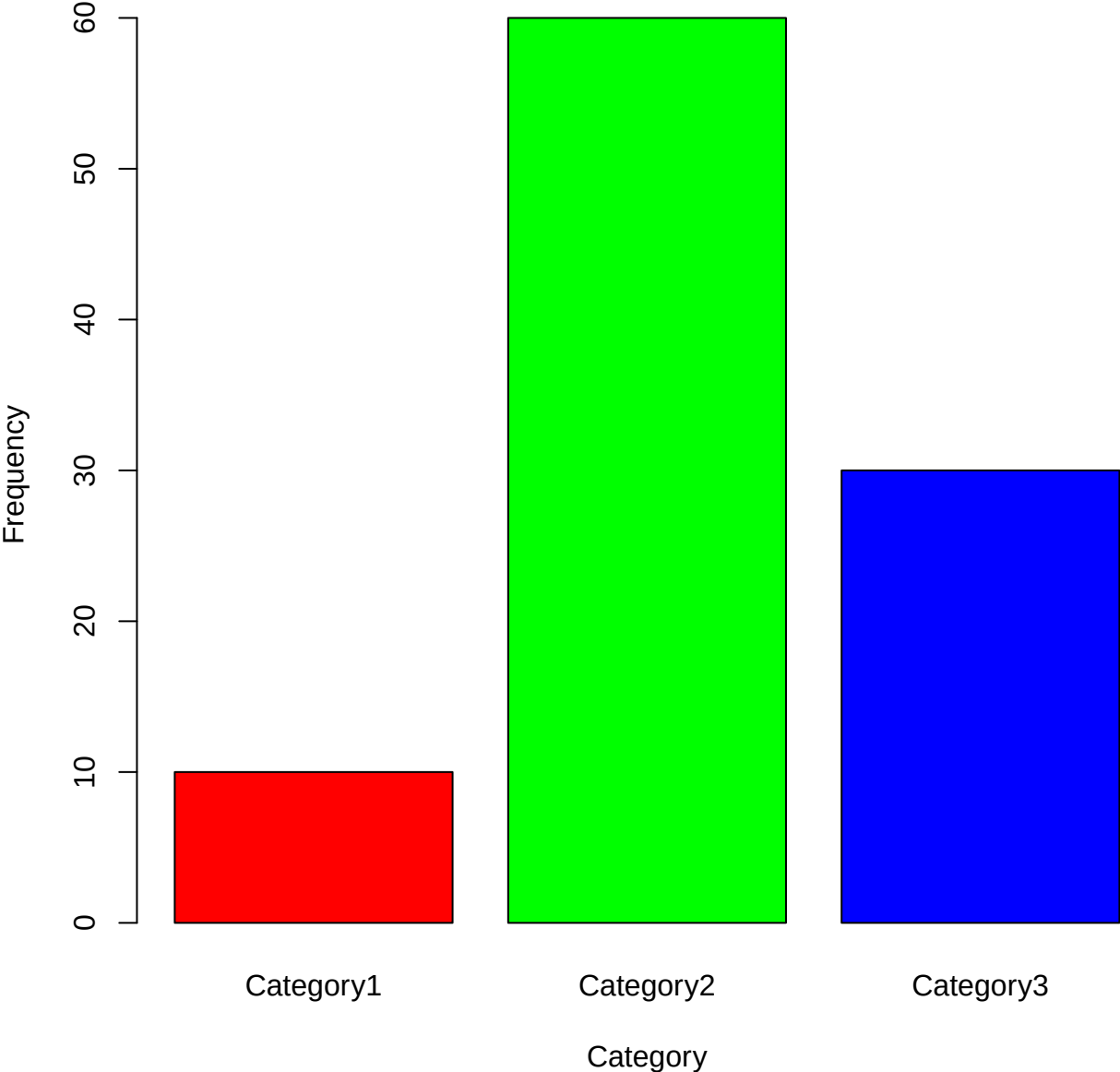
CategoryVariable
