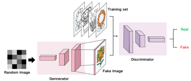
Figure 1: GANs principle.
