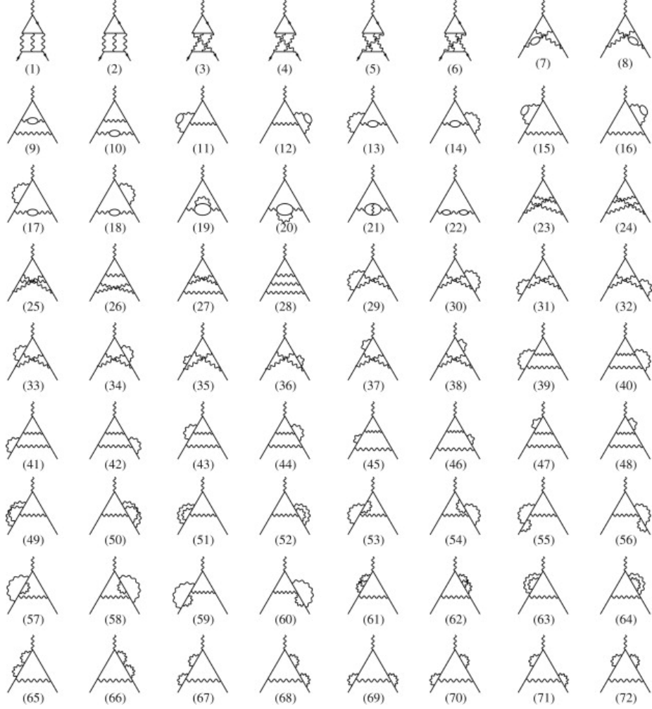
Figure 1.2: The three-loop vertex diagrams contributing to a_1^{(6)} magnetic moment (from Jegerlehner and Nyffeler [110]). Lautrup et al. [140] were the first to note that subsets (3, 0, 0) = \{23, 24, 25, 26, 27, 28\} ; (2, 1, 0) = \{29, 31, 33, 35, 37, 39, 41, 43, 45, 47\} and its time-reversal (2, 0, 1) = \{30, 32, 34, 36, 38, 40, 42, 44, 46, 48\} ; (1, 2, 0) = \{49, 51, 53, 55, 57, 59, 61, 63, 65, 67\} and its time-reversal (1, 0, 2) = \{50, 52, 54, 56, 58, 60, 62, 64, 66, 68\} ; and (1, 1, 1) = \{69, 70, 71, 72\} are the minimal gauge sets, see figure 1.4.
