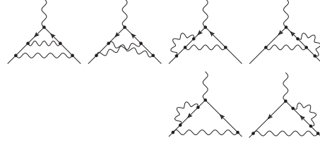
Figure 1.1: The two-loop vertex diagrams contributing to a^{(4)}[V] magnetic moment anomaly. From Volkov [198].
