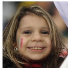
Attribute-only (Ours)
