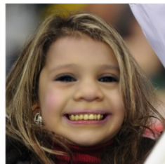
Identity-only
