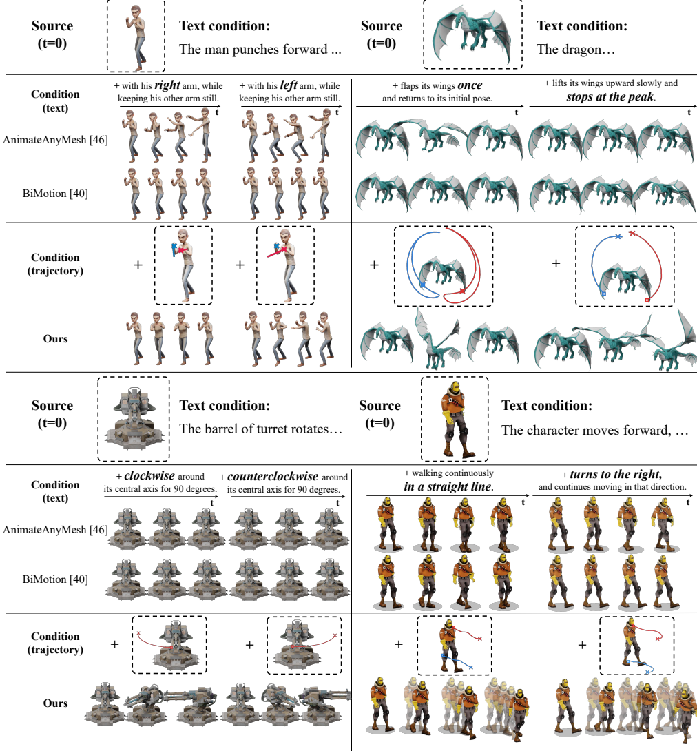
Figure 3: Qualitative comparison with text-based baselines. The baselines [40, 46] are conditioned on a pair of text prompts describing different specific motion details, while our model is guided by sparse trajectories representing those details. Our model uses only the visualized trajectories as inputs—at most two per example. By providing direct spatial cues, our method faithfully generates the intended motion, whereas the text-conditioned baselines fail to produce expressive motions aligned with the text and show little meaningful difference across the varying prompts. We provide video results in our supplementary materials.
