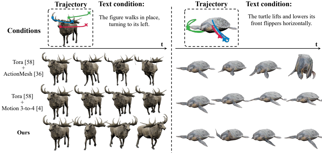
Figure 4: Qualitative comparison with video-based baselines. We compare our method against baselines that we construct by combining controllable video generation [58] with video-based dynamic 3D generation [4, 36]. These baselines take 2D trajectories projected onto the given camera view as input. The constructed pipelines fail to synthesize dynamic 3D shapes that faithfully follow the trajectory guidance and struggle to preserve the visual structure of the input shape during motion.
