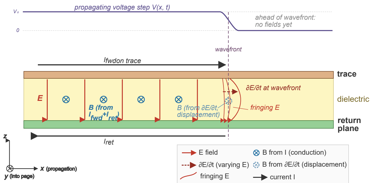
Side view of microstrip \mathbf{E} and \mathbf{B} fields along the propagation direction.
