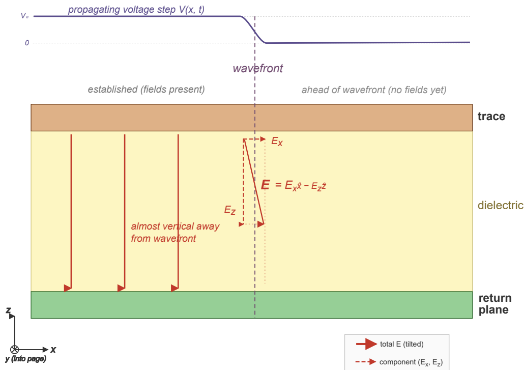
Microstrip electric field components.
