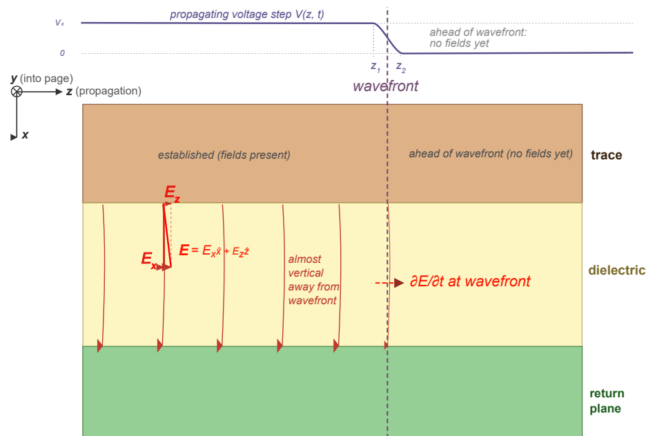
Microstrip electric field.
