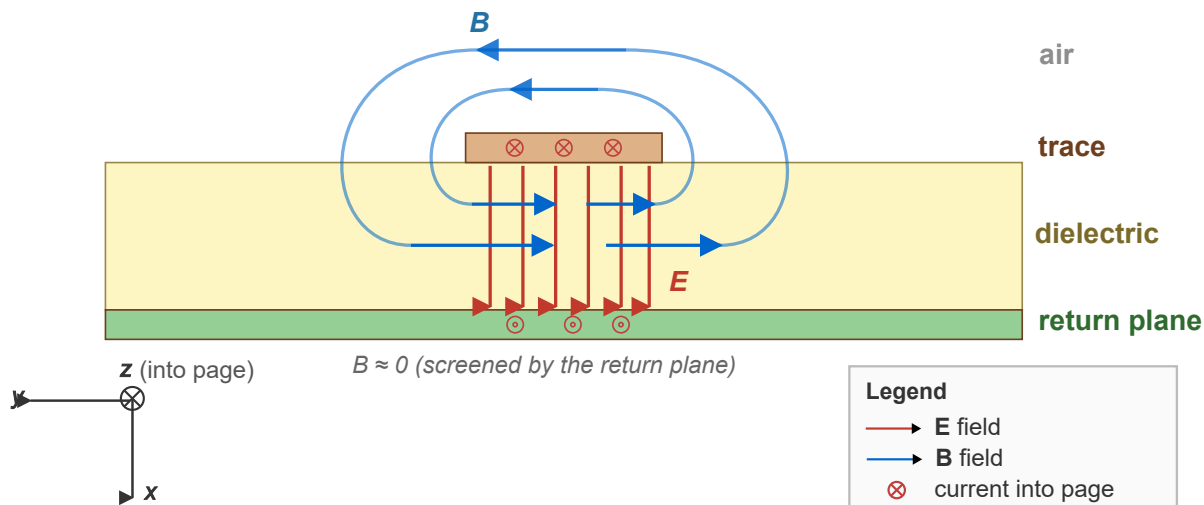
Cross-section of the microstrip. \mathbf{B} -field curls around the trace.
