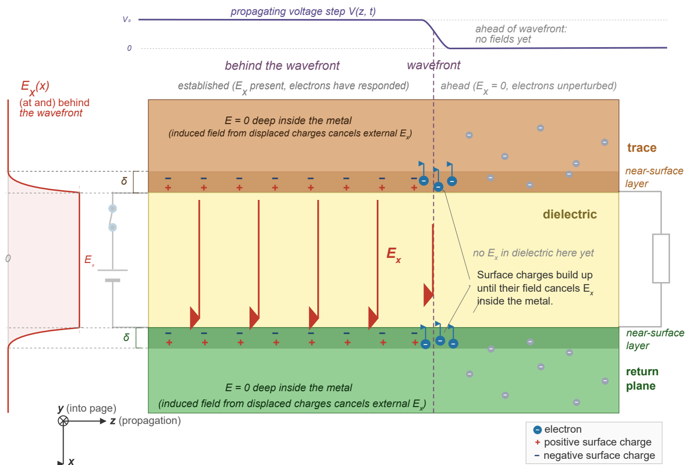
Microstrip E_x confinement.
