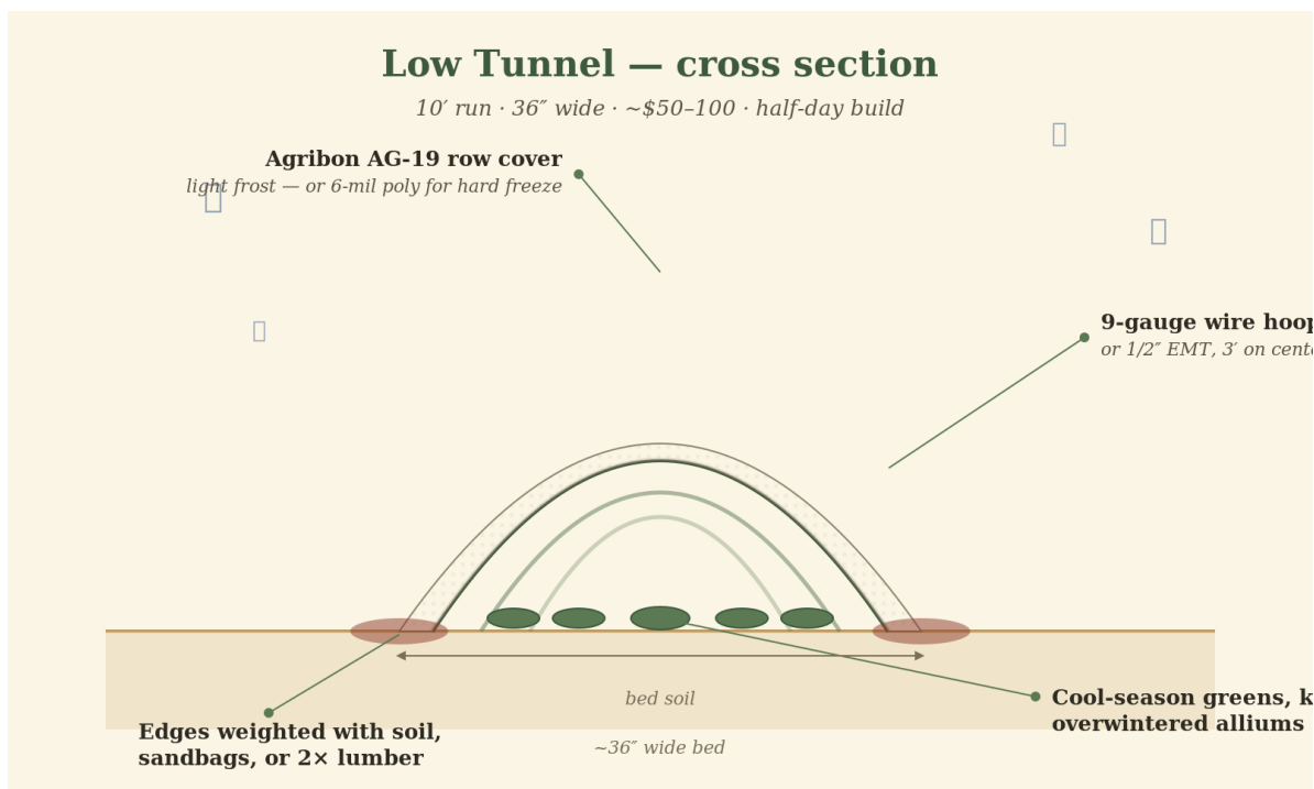
Figure 3: Cross section of a low tunnel over a 36" wide bed. Hoops on 3 ft centers; cover edges weighted with soil or 2x lumber. Use row cover for light frost (down to 26 °F); switch to 6-mil poly for hard freezes.
