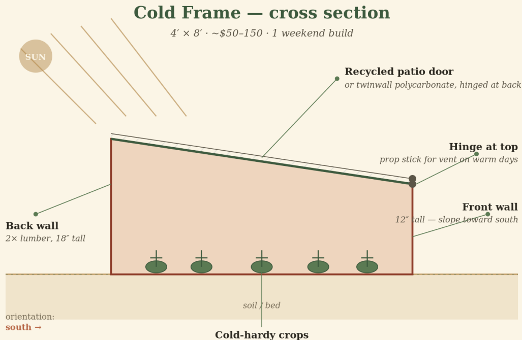
Figure 2: Cross section of the 4×8 ft cold frame. The back wall is taller than the front so the lid slopes toward the south, maximizing winter solar gain and shedding precipitation away from the structure.
