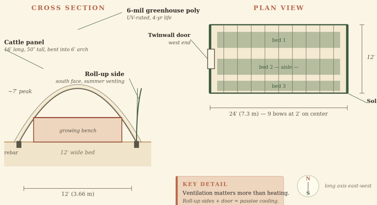
Figure 4: Hoop house 12×24 — the cattle-panel-arch design. Cross section (left) shows the bow profile, growing bench, roll-up side, and rebar anchors. Plan view (right) shows 9 bows on 2 ft centers, end-wall door on the west, and three growing beds inside. Orient the long axis east-west for maximum winter solar gain.
