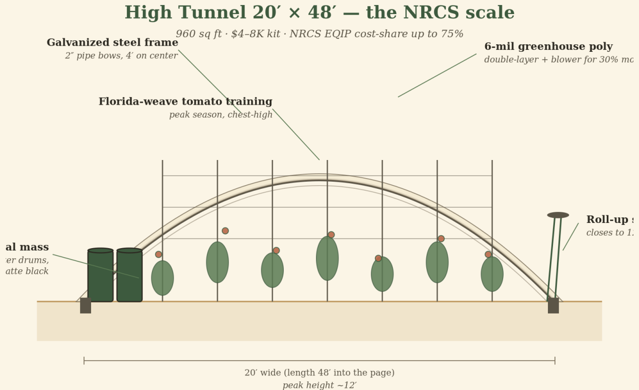
Figure 5: High tunnel 20×48 — the NRCS-scale structure. Galvanized steel bows on 4 ft centers, double-layer 6-mil greenhouse poly, roll-up sides on both long sides, twin-wall end walls. Florida-weave tomatoes shown at peak season; 55-gal water drums against the north wall serve as thermal mass.
