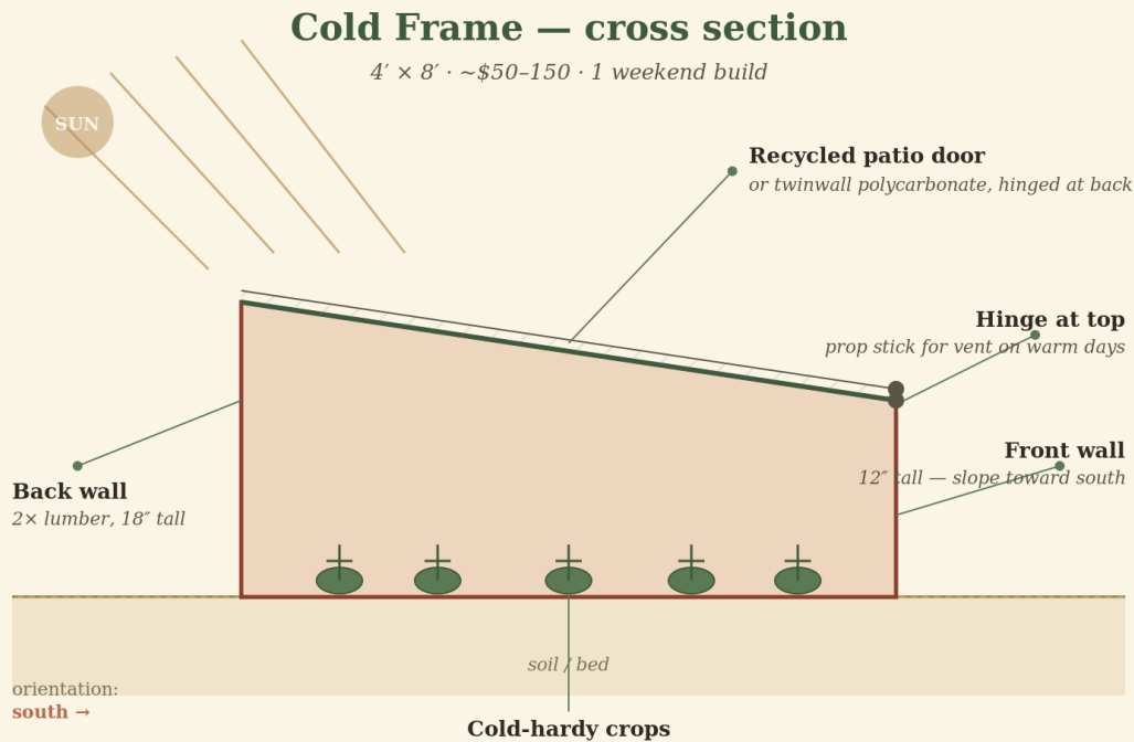
Figure 2: Cross section of the 4×8 ft cold frame. The back wall is taller than the front so the lid slopes toward the south, maximizing winter solar gain and shedding precipitation away from the structure.
