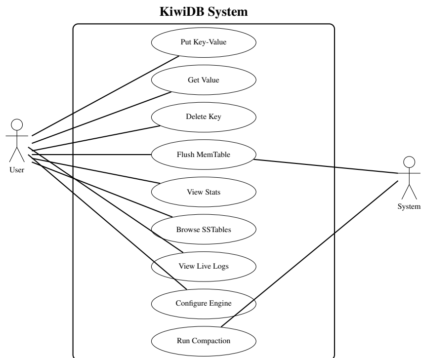
Figure 4.5: Use Case Diagram for KiwiDB.
