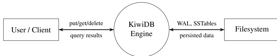
Figure 4.2: DFD Level 0 — Context Diagram.
