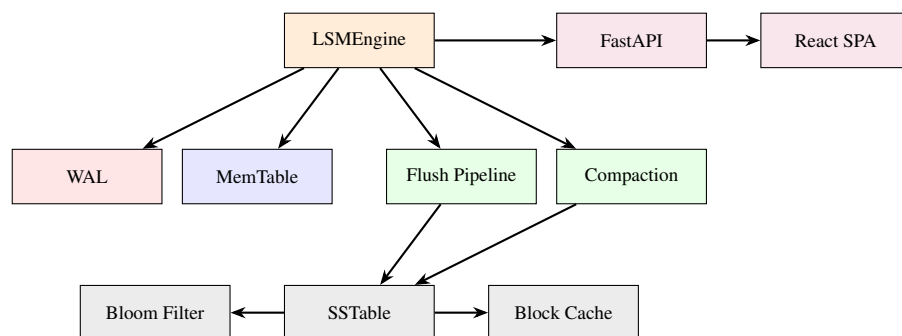
Figure 4.9: Component Diagram.
