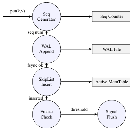
Figure 4.4: DFD Level 2 — Write path detail.
