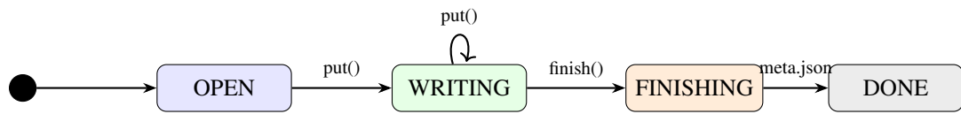
Figure 4.11: State Machine Diagram — SSTableWriter lifecycle.
