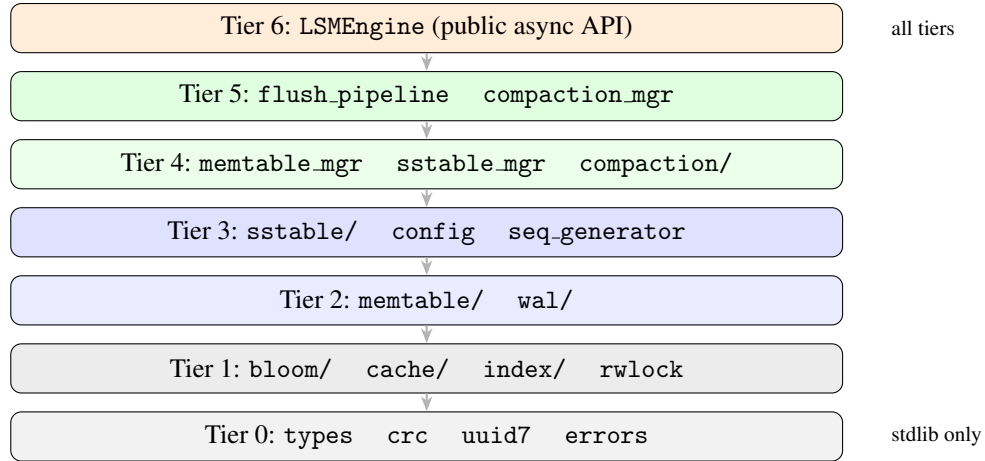
Figure 4.1: KiwiDB layered architecture. Each tier depends only on tiers below it.
