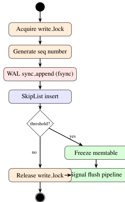
Figure 4.6: Activity Diagram — Write Path.
