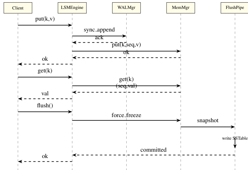
Figure 4.7: Sequence Diagram — Put, Get, and Flush operations.
