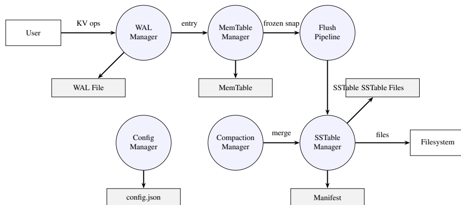
Figure 4.3: DFD Level 1 — Major subsystems and data stores.
