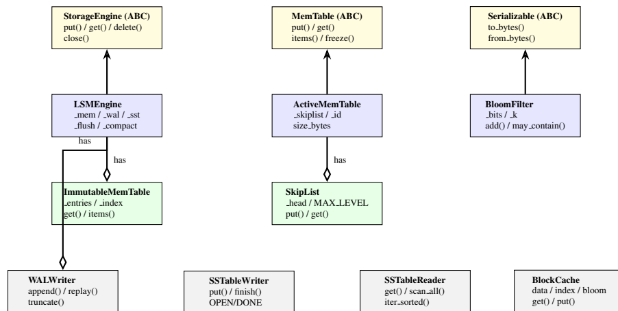
Figure 4.8: Class Diagram — Core class hierarchy.
