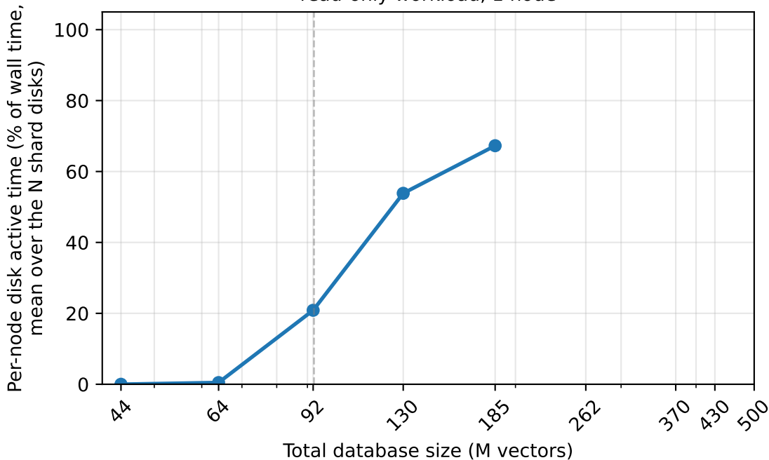
Per-node SSD active time vs. database size read-only workload, 1 node
