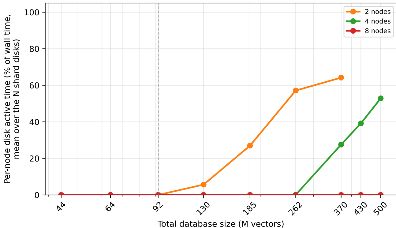
Per-node SSD active time vs. database size read-only workload, 2/4/8 nodes
