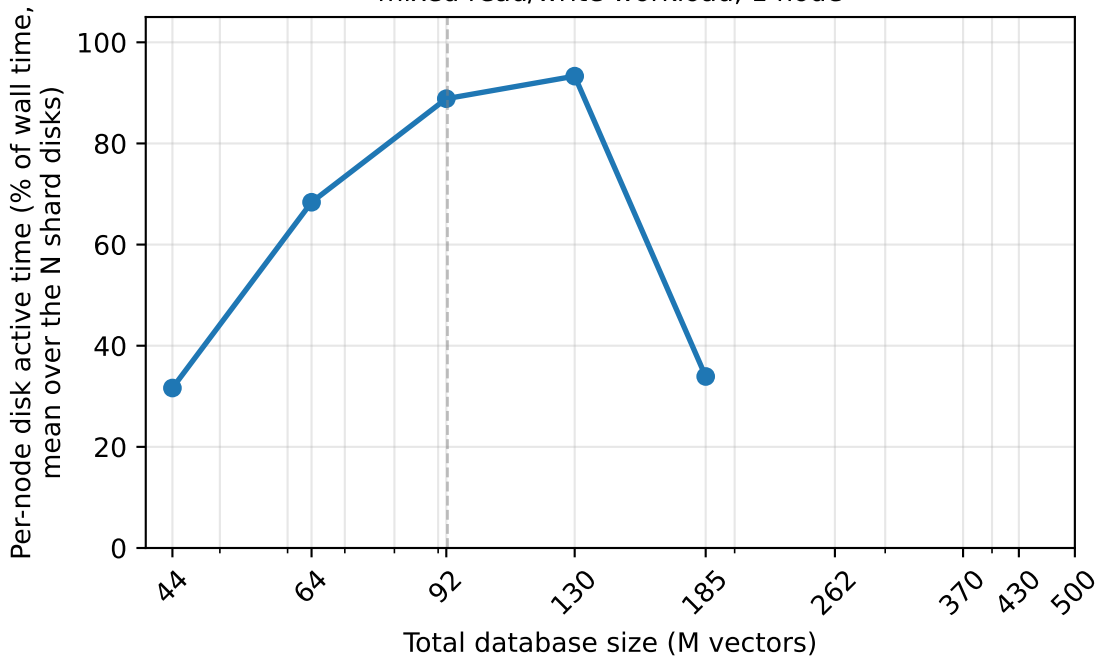
Per-node SSD active time vs. database size mixed read/write workload, 1 node
