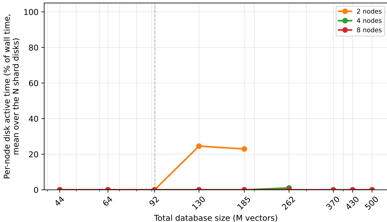
Per-node SSD active time vs. database size mixed read/write workload, 2/4/8 nodes
