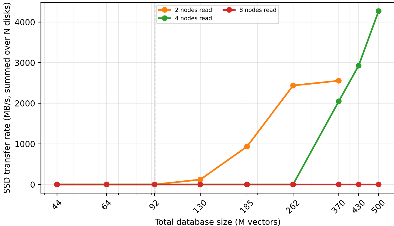
Aggregate SSD transfer rate vs. database size read-only workload, 2/4/8 nodes
